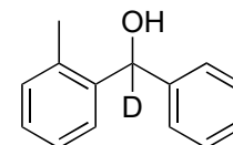
α-Deutero- o -methyl-benzhydrol ( 2 ) 1 H NMR (400 MHz, CDCl 3 )
